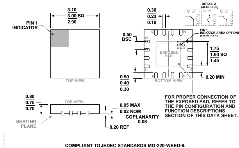
Figure 47. 16-Lead Lead Frame Chip Scale Package [LFCSP]
