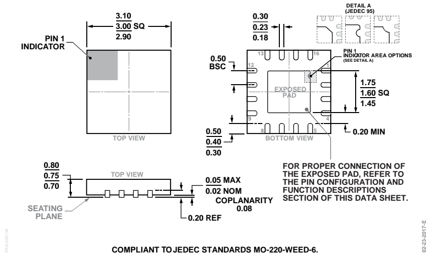
COMPLIANT TO JEDEC STANDARDS MO-220-WEED-6. Figure 47. 16-Lead Lead Frame Chip Scale Package [LFCSP] 3 mm × 3 mm Body and 0.75 mm Package Height (CP-16-22) Dimensions shown in millimeters
