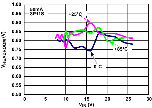
FIGURE 12. V_{HEADROOM} vs V_{IN} vs TEMPERATURE AT 50mA
