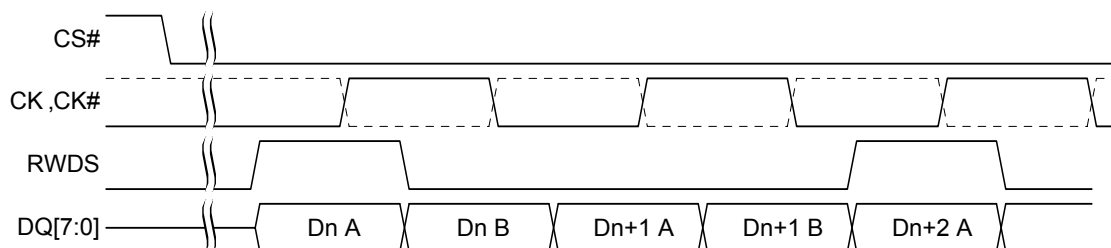
Figure 11.3 Data Placement During a Write Transaction
