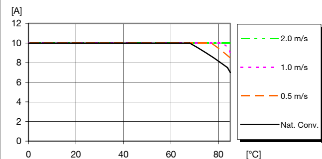
Available load current vs. ambient air temperature and airflow at V_I = 12.0 V , V_{OUT} = 5.0 V . See Thermal Consideration section.
