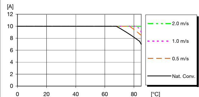
Available load current vs. ambient air temperature and airflow at V_I = 12.0\text{ V} , V_{OUT} = 5.0\text{ V} . See Thermal Consideration section.
