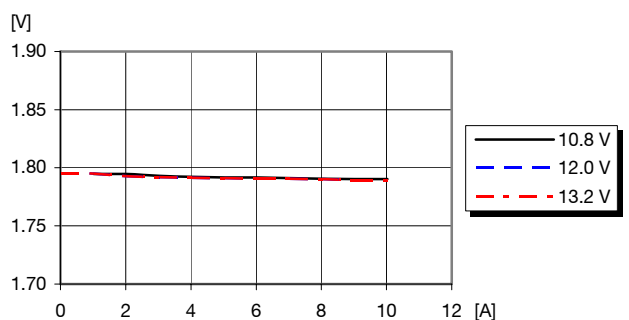
Output voltage vs. load current at T_{ref} = +25^{\circ}C
