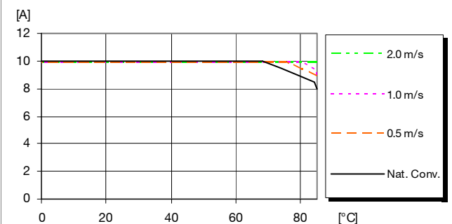
Available load current vs. ambient air temperature and airflow at V_I = 12.0\text{ V} , V_{OUT} = 1.8\text{ V} . See Thermal Consideration section.
