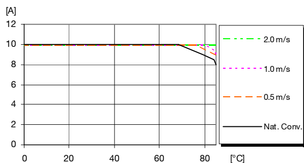
Available load current vs. ambient air temperature and airflow at V_I = 12.0\text{ V} , V_{OUT} = 1.8\text{ V} . See Thermal Consideration section.
