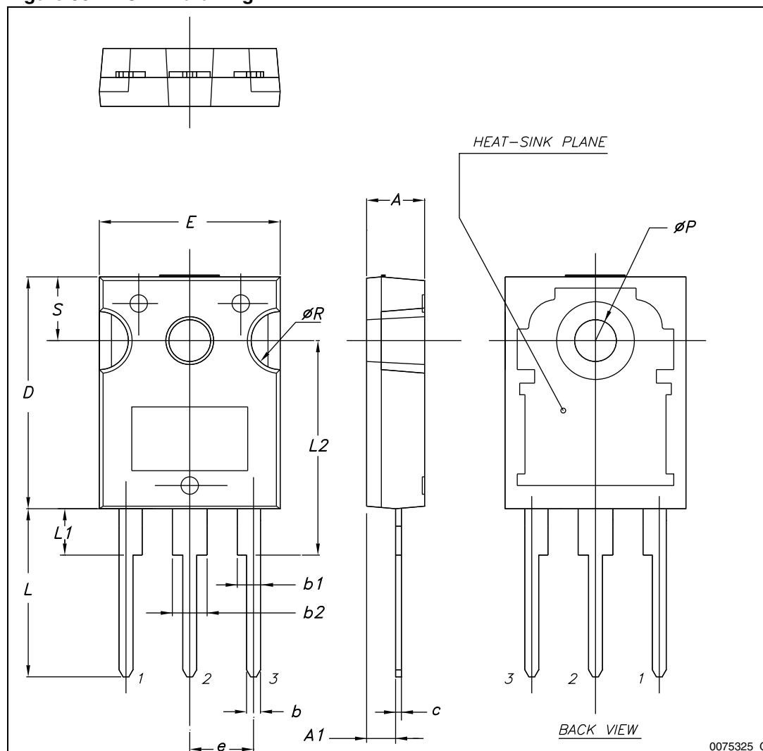
Figure 30. TO-247 drawing
