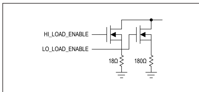
Figure 7. Electronic Load Block Diagram
