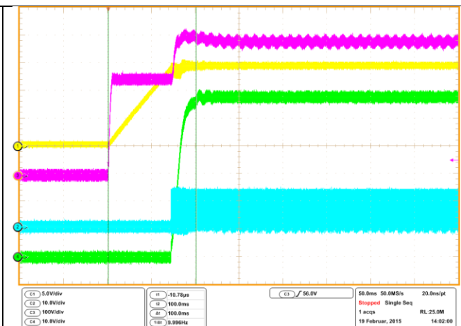
Figure 7: AC Input Voltage 230V ACIN , Full Load
