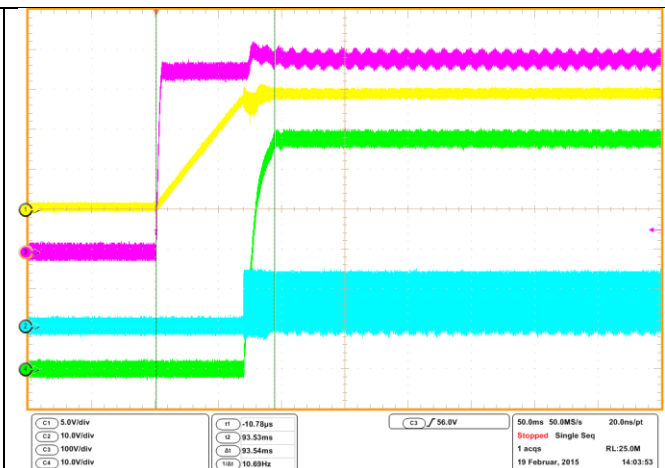
Figure 9: AC Input Voltage 300V ACIN , Full Load
