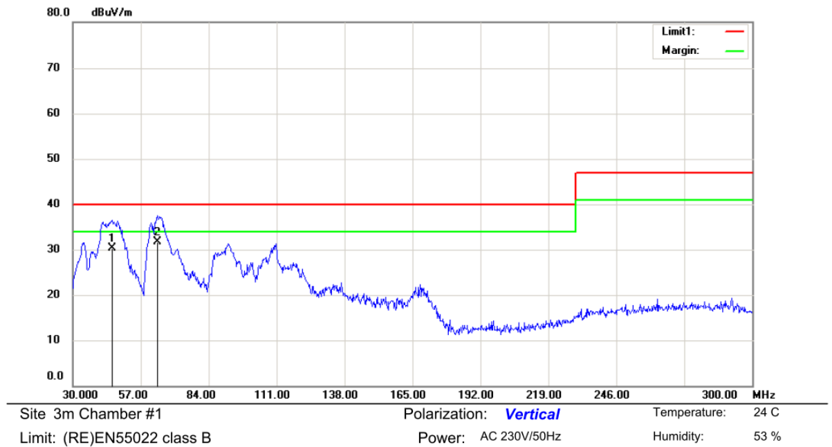
Figure 25 Radiated EMI -- 230VAC/50Hz Vertical
