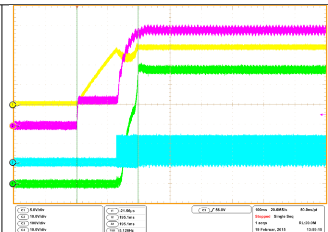
Figure 5: AC Input Voltage 85V ACIN , Full Load
