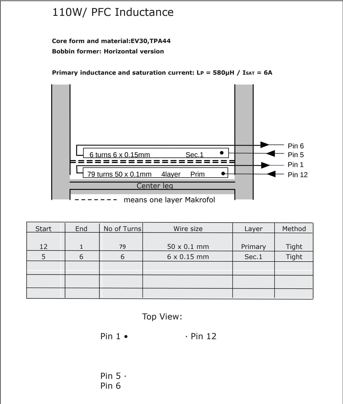
Figure 29 PFC Choke
