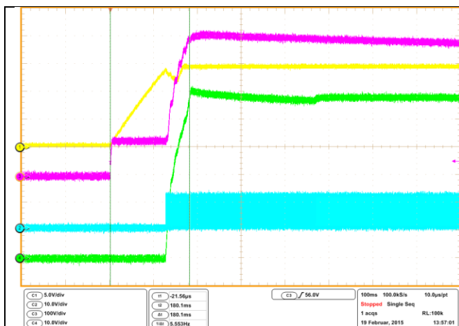
Figure 4: AC Input Voltage 85V ACIN , NO Load
