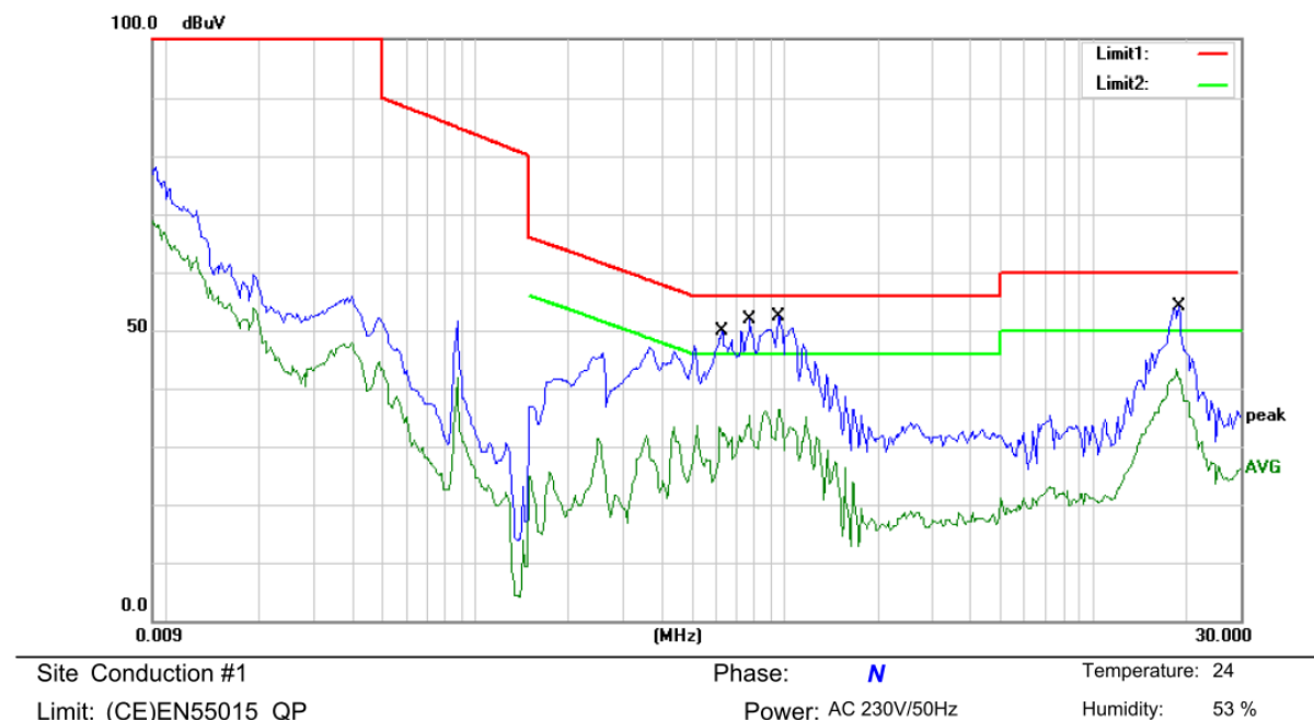
Figure 20 Conducted EMI -- 230VAC/50Hz N
