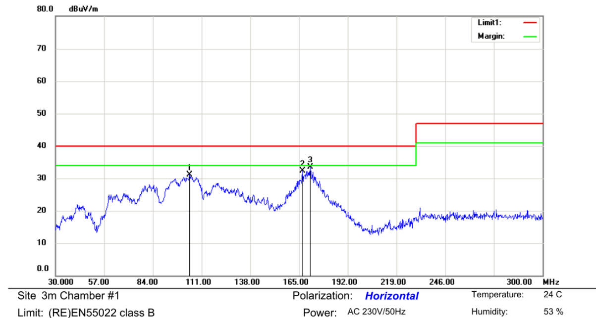
Figure 24 Radiated EMI -- 230VAC/50Hz Horizontal
