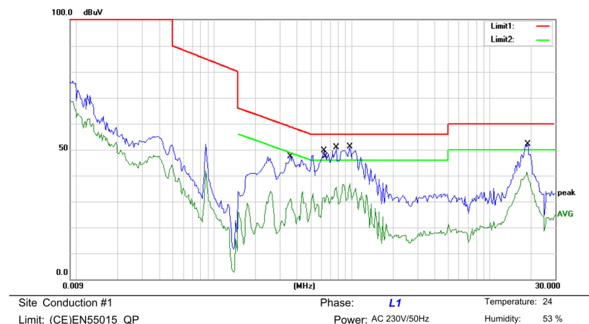
Figure 21 Conducted EMI -- 230VAC/50Hz L
