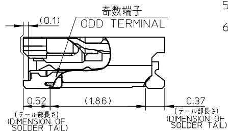
SECTION X-X
