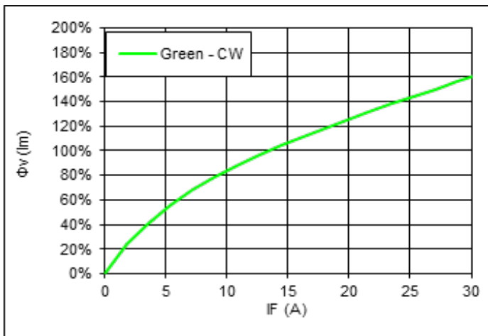
Relative Output Flux vs. Forward Current 1
