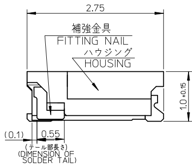
SECTION Y-Y
