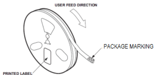
Figure 13: Reel Orientation
