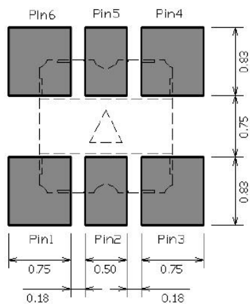
Figure 12: Recommended Solder Pad (Units: mm)
