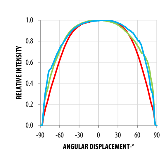
Figure 5: Radiation Pattern
