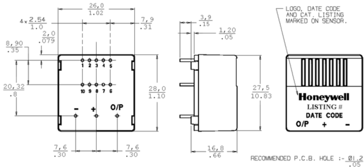
Mounting Dimensions - for reference only (mm/in)
