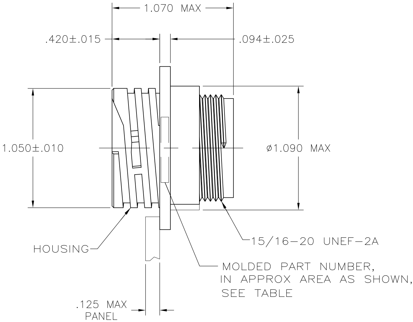
DETAIL A
