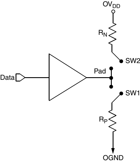
Figure 77. Driver Impedance Measurement
