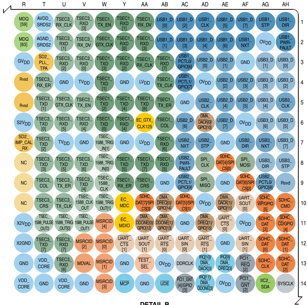
DETAIL B
