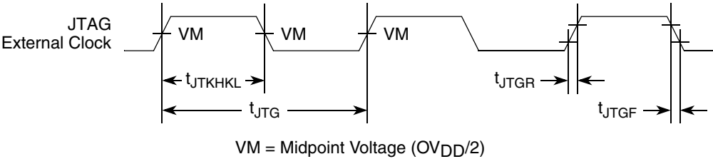
Figure 46. JTAG Clock Input Timing Diagram
