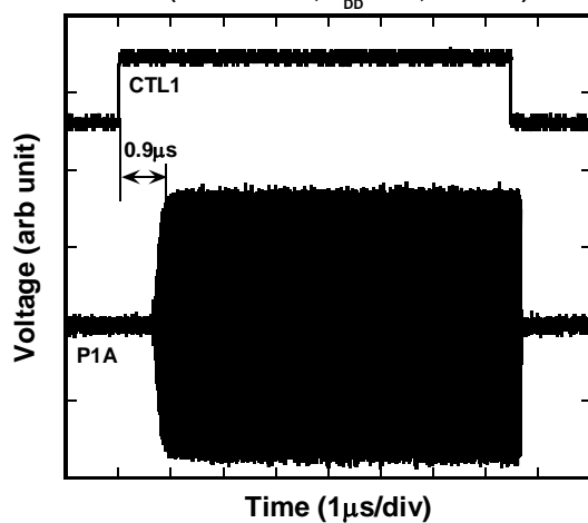
Switching Time
