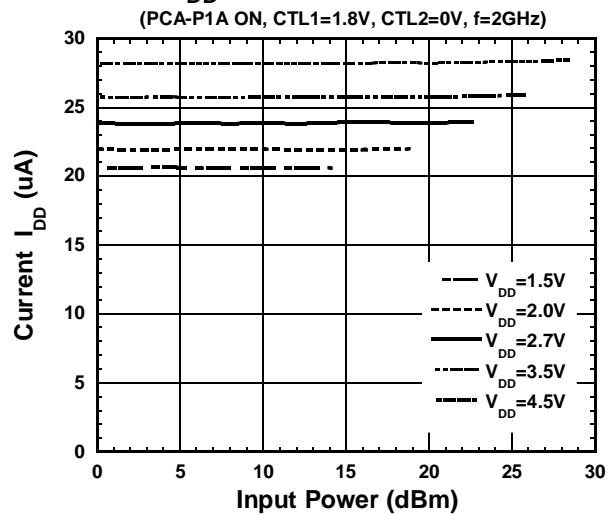
I_{DD} vs. Input Power
