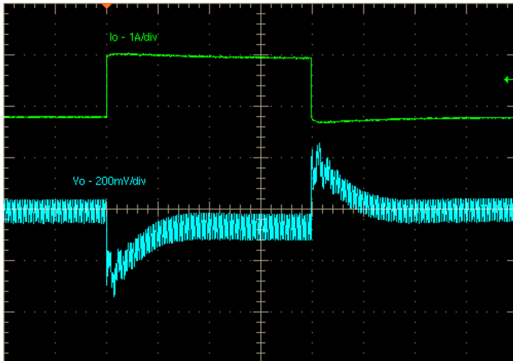
Figure 6. Load Transient Response (10A/μs)
