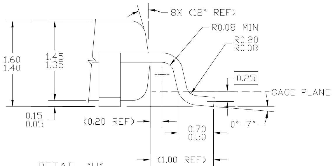
DETAIL "H"
