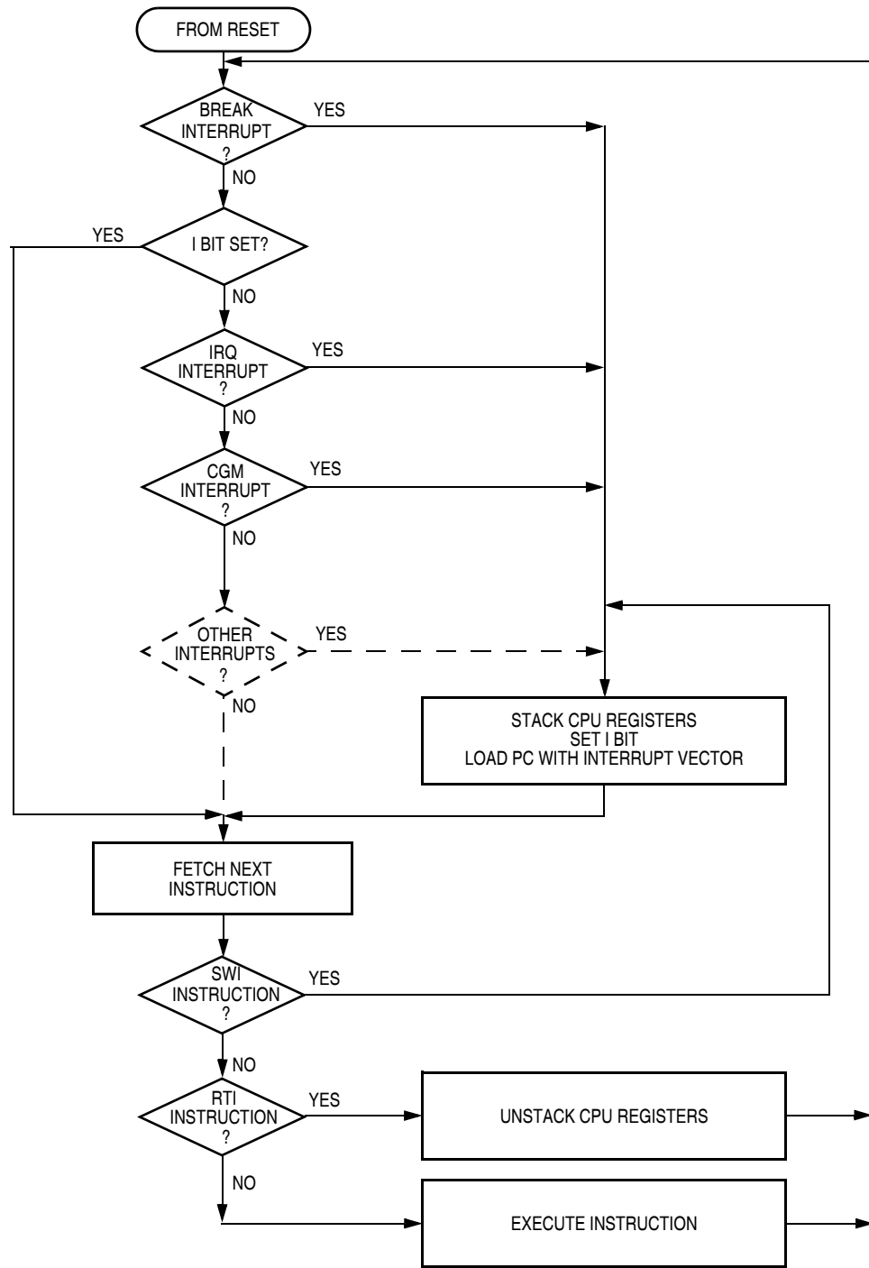
Figure 14-10. Interrupt Processing
