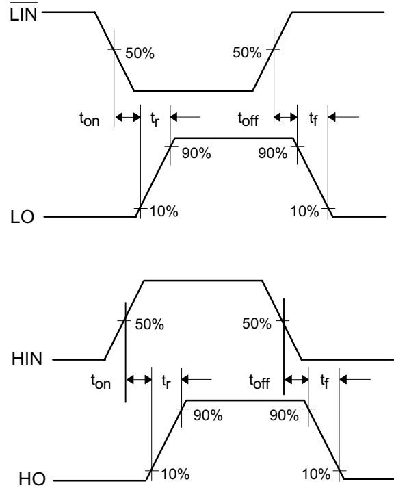
Figure 2. Switching Time Waveform Definitions
