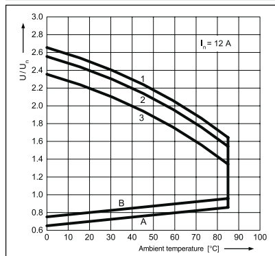
Coil operating range - DC - standard version
