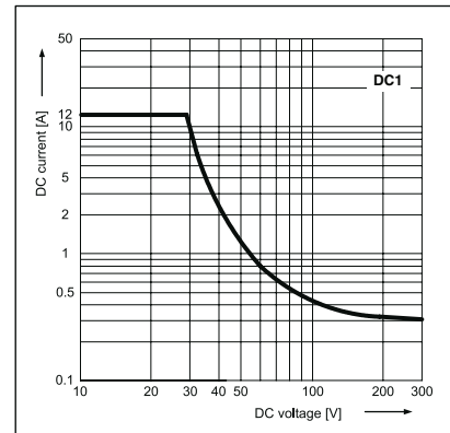
Max. DC resistive load breaking capacity - standard version
