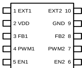
MSOP-10 (TOP VIEW)
