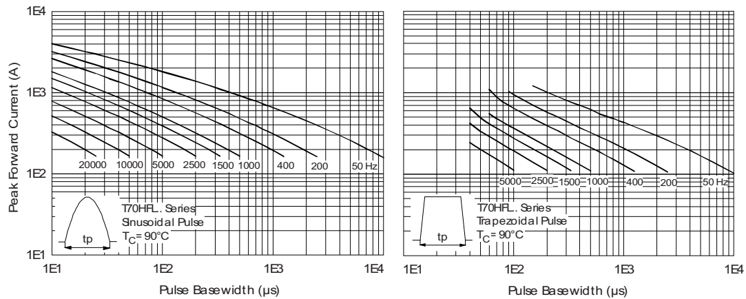
Fig. 41 - Frequency Characteristics
