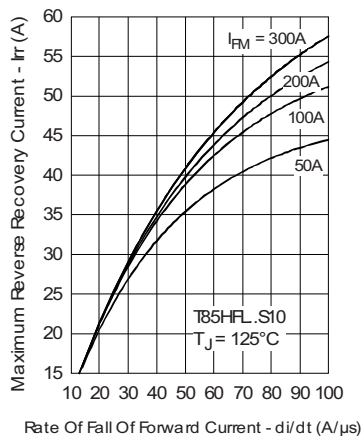
Fig. 36 - Recovery Current Characteristics
