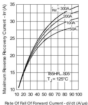
Fig. 33 - Recovery Current Characteristics
