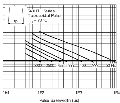
Fig. 37 - Frequency Characteristics
