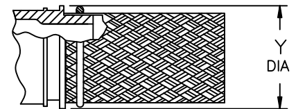
TINEL-LOCK TERMINATION
