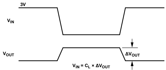
Figure 21. Charge Injection
