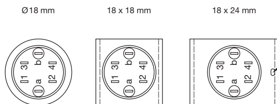
Component layout 4
