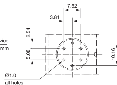
Drilling plan (solder side)
