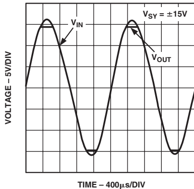
Figure 3b. Input Voltage Can Exceed the Supply Voltage Without Damage
