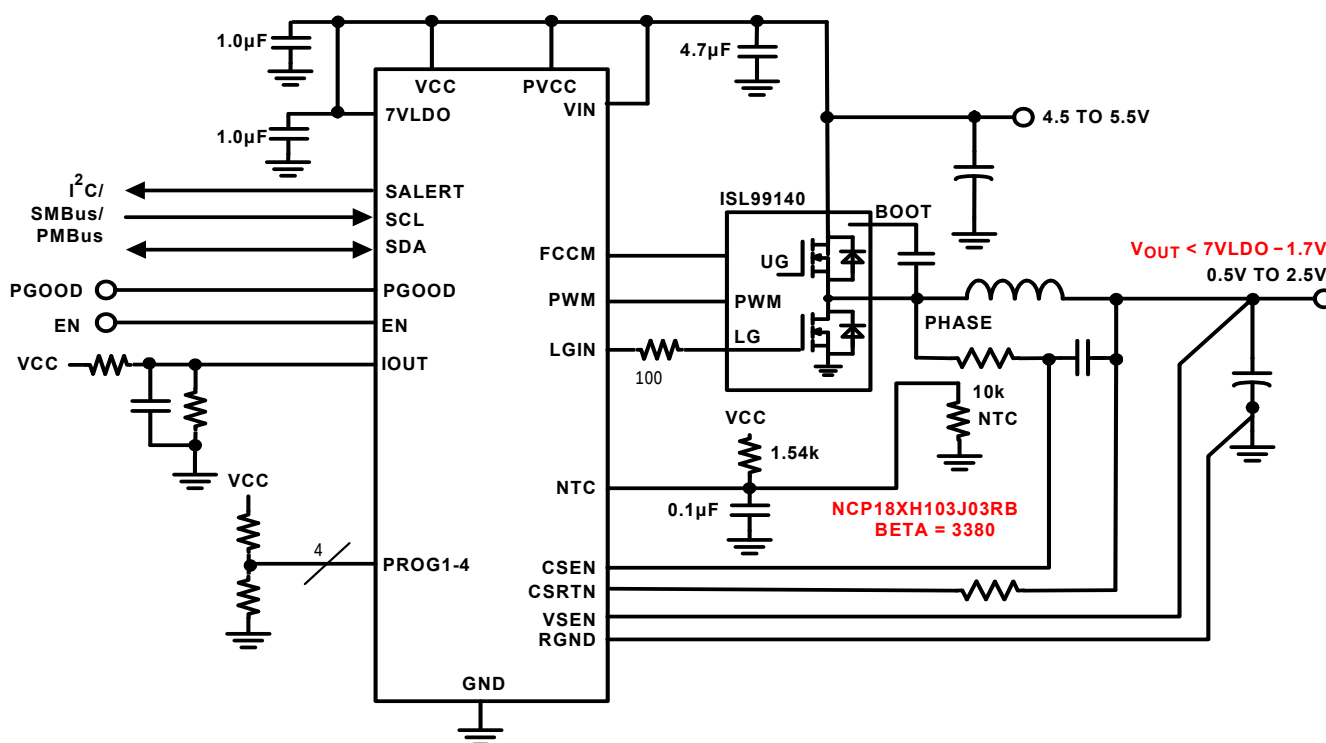
FIGURE 2. 5V INPUT APPLICATION
