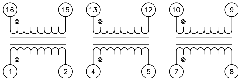
SCHEMATIC
