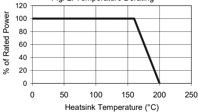
Fig. 2: Temperature Derating
