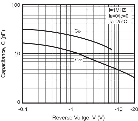
Fig.6 - C_{ob}/C_{ib} — V_{CB}/V_{EB}
