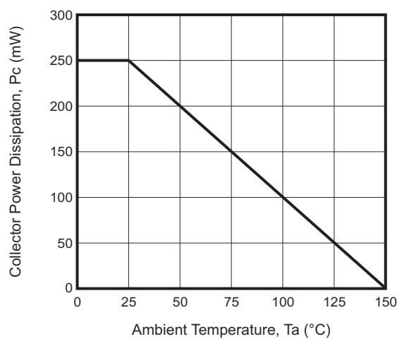
Fig.7 - P_c — T_a
