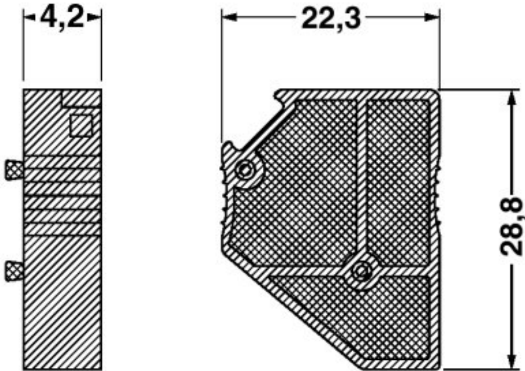
Dimensional drawing
