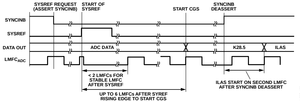
Figure 66. JESD204B Tx Resynchronization Timing
