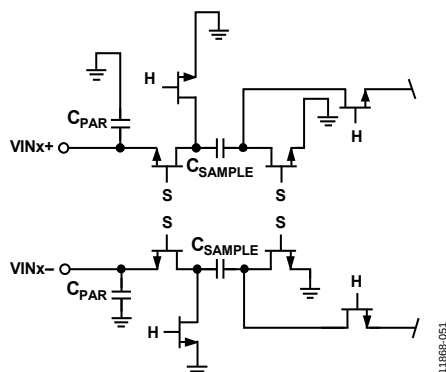
Figure 46. Switched-Capacitor Input Circuit
