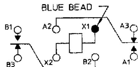
TERMINAL VIEW
