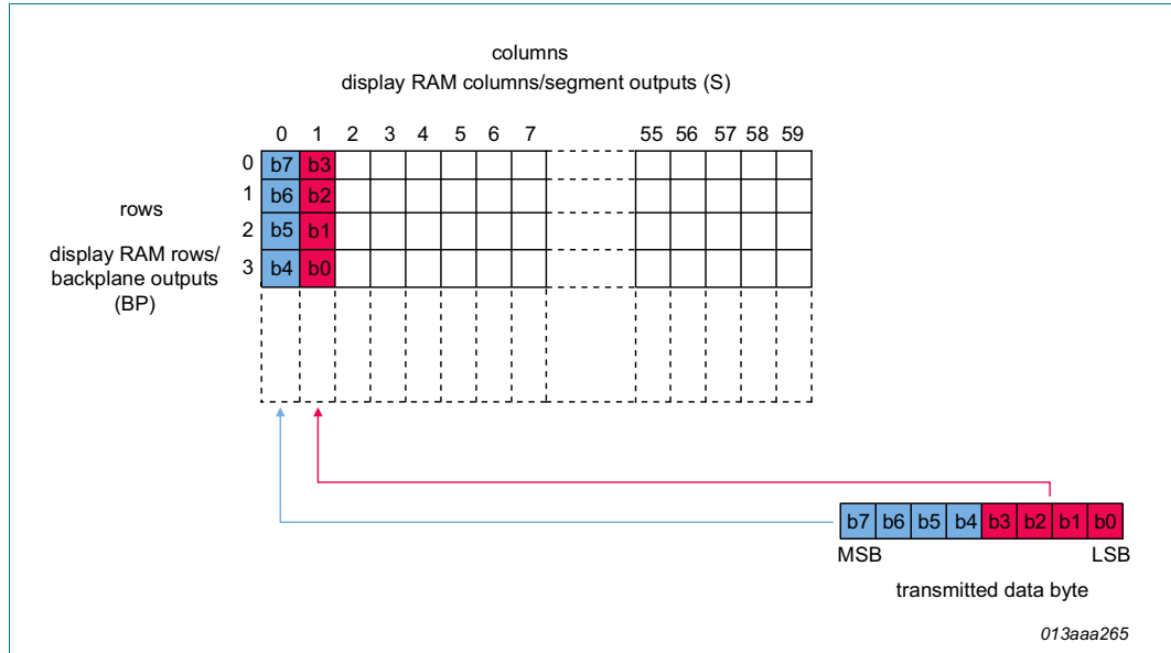
Fig 31. Display RAM filling order in 1:4 multiplex drive mode
