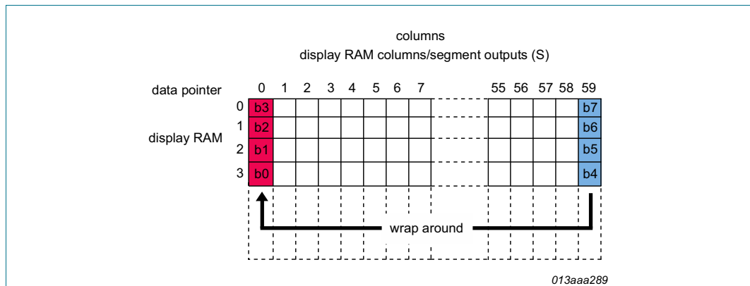
Fig 32. Data pointer wrap around in 1:4 multiplex drive mode
