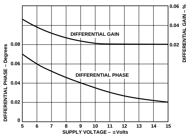
Figure 2. Differential Gain and Phase vs. Supply Voltage, Gain = +2, R_L = 150 \Omega
