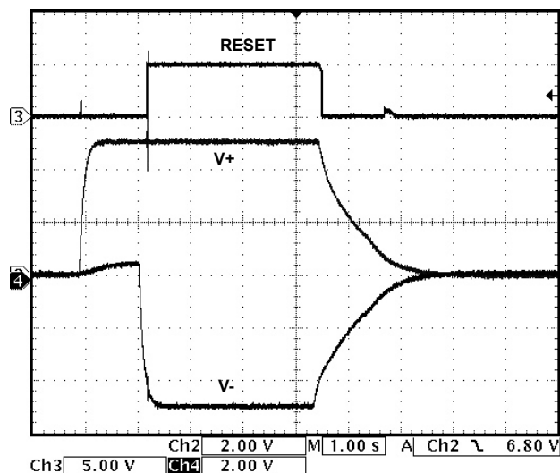
FIGURE 16. ±5V MONITORING
