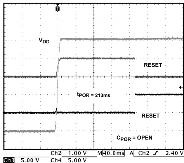
FIGURE 10. RESET AND \overline{\text{RESET}} ASSERTION
