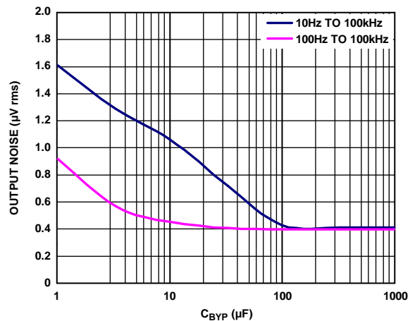
Figure 45. RMS Noise vs. C_{BYP}
