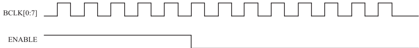
ENABLE Timing Diagram
