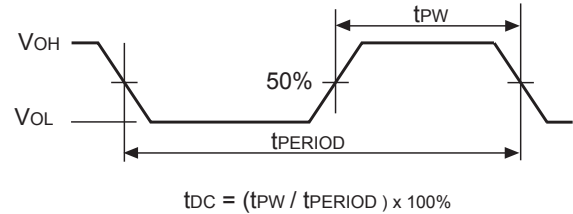
Duty Cycle – t_{DC}
