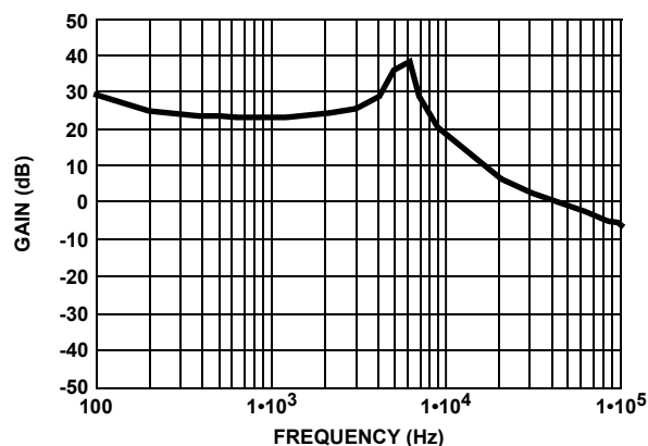
FIGURE 31A. PREDICTED LOOP GAIN
