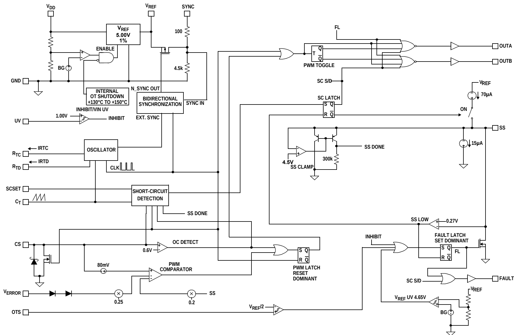
FIGURE 2. ISL6741 FUNCTIONAL BLOCK DIAGRAM
