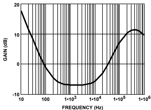
FIGURE 29A. IDEAL ERROR AMPLIFIER GAIN
