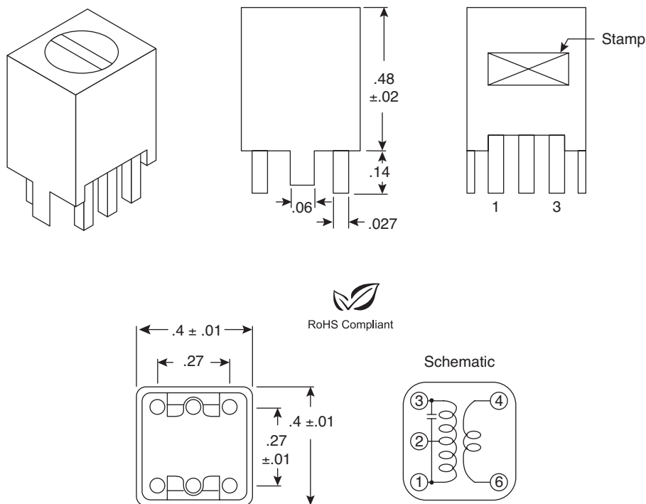
Dimensions (in.)
