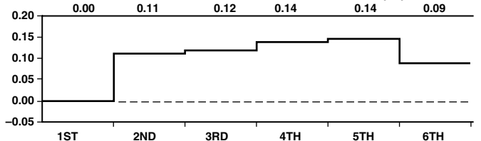
TPC 15. Composite Output Differential Phase and Gain, PAL
