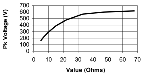
IEC61000-4-5 1.2/50μs Pulse
