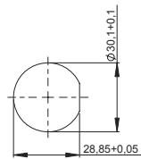
Drilling diagram
