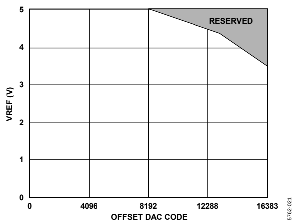
Figure 22. Offset DAC Code Range
