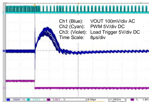
Figure 4-6 15 to 5A Load Step – Max. Capacitance
