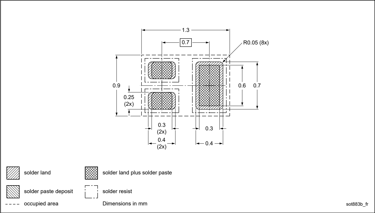
Fig. 10. Reflow soldering footprint for DFN1006B-3 (SOT883B)
