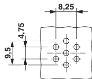
Drilling diagram
