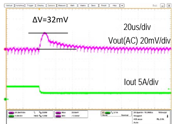
Step Load Transient Response (Vin=5.0V, Vout=1.0V, Cload=400uF, Iout=6A to 3A, 2.5A/us)
