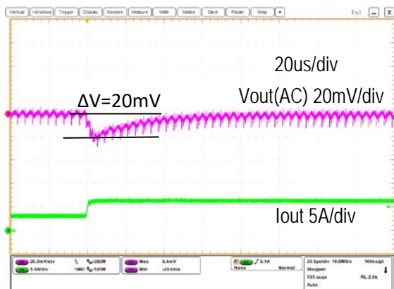
Step Load Transient Response (Vin=5.0V, Vout=1.0V, Cload=400uF, Iout=3A to 6A, 2.5A/us)
