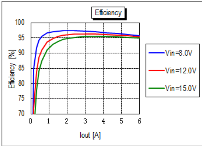
Efficiency vs. Line Voltage and Load Current @ +25degC. (Vout = 5.0V)
