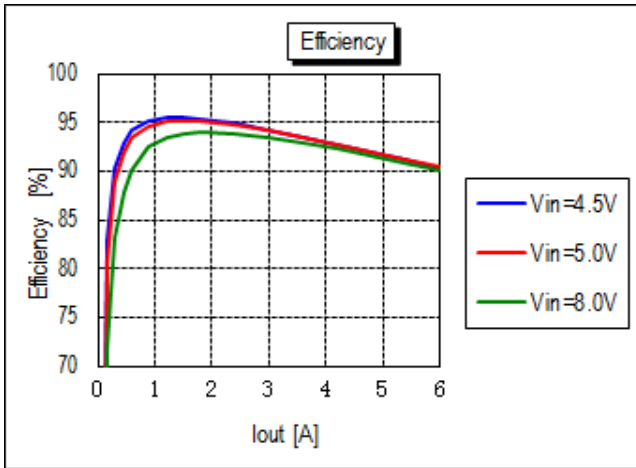
Efficiency vs. Line Voltage and Load Current @ +25degC. (Vout = 1.8V)
