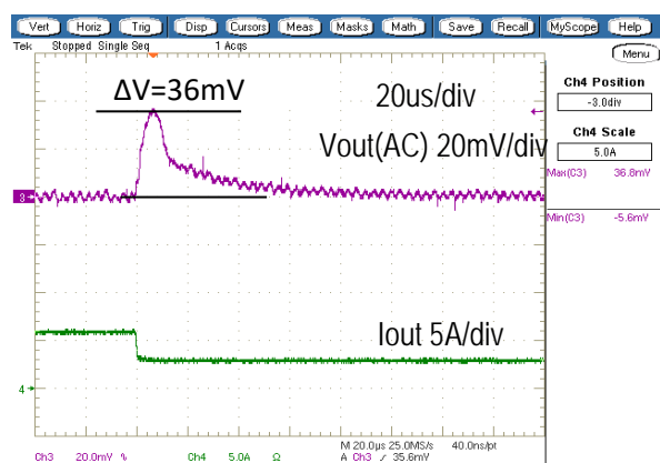
Step Load Transient Response (Vin=12V, Vout=1.0V, Cloud=400uF, Iout=6A to 3A, 2.5A/us)
