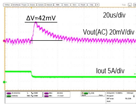
Step Load Transient Response (Vin=5.0V, Vout=0.7V, Cload=400uF, Iout=6A to 3A, 2.5A/us)
