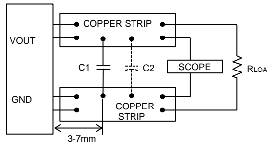
C1=220uF x 2 or 100uF x 4 CERAMIC C2=OPEN Figure: Measuring Output Ripple and Noise
