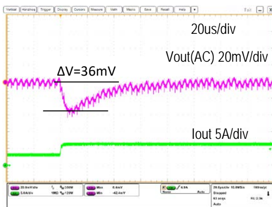
Step Load Transient Response (Vin=5.0V, Vout=0.7V, Cload=400uF, Iout=3A to 6A, 2.5A/us)
