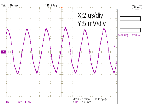
Output Ripple and Noise (Vin=12V, Vout=5.0V, Iout=6A, Cload=400uF, ScopeBW=20MHz)
