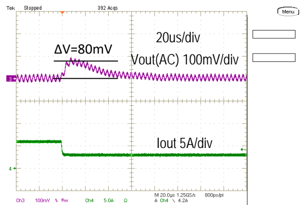
Step Load Transient Response (Vin=12V, Vout=5.0V, Cload=400uF, Iout=6A to 3A, 2.5A/us)
